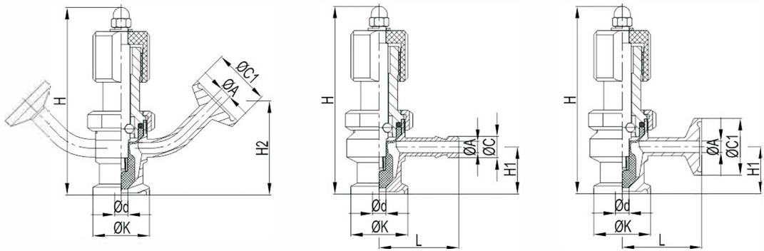
卡箍型无菌取样阀(SGM) Clamped Aseptic Sample Valve(SGM)
